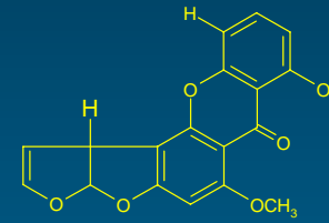
Sterigmatocystin
