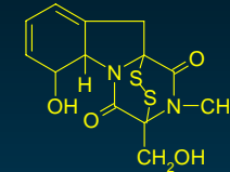
Gliotoxin
