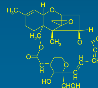
Satratoxine
